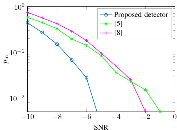
Fig. 5: Probability of missed detection (for \alpha = 0.05 ) for the following scenario: P = 4.2 , S = 192 symbols, L = 2 antennas, M = 25 realizations, P_{\max} = 10 , and D = 20
