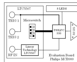
Fig. 4. Trigger components.
