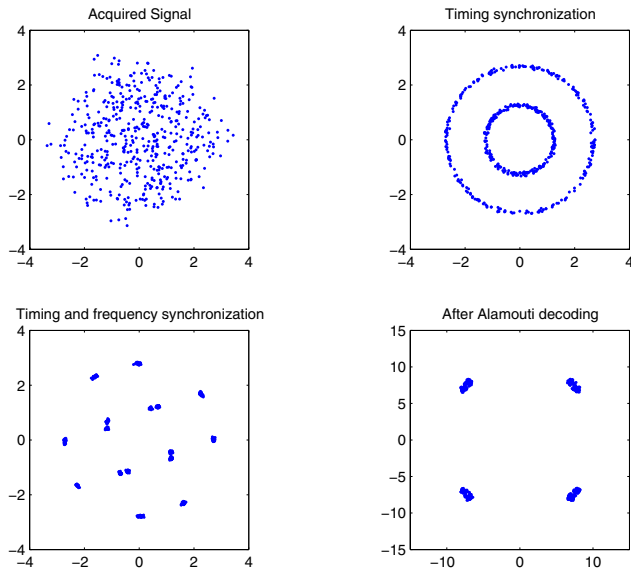
Fig. 7. Symbol constellations at the receiver.
