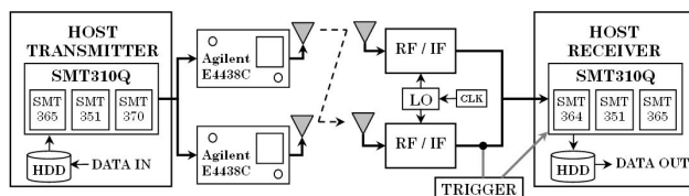
Fig. 1. Schematic diagram of the 2 \times 2 MIMO platform.
