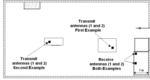
Fig. 6. Locations of the TX's and RX's in the two experiments.
