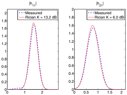
Fig. 11. PDF of two channel coefficients for the second experiment.
