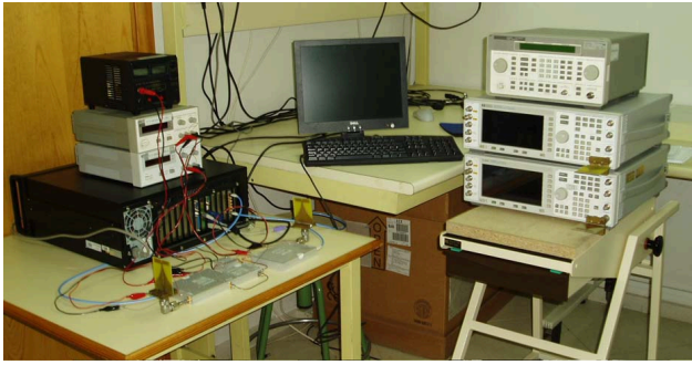
Fig. 2. A picture of the of the 2 \times 2 MIMO platform.
